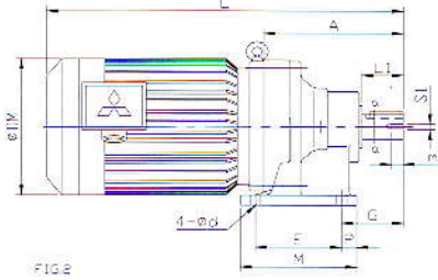
Fig 2. Type CNHM (3~5 HP) (Grease Lubrication)
