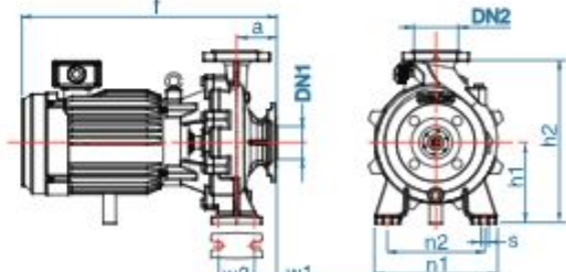
WCM-3705FS,FT
