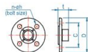
FLANGE DIMENSIONS (mm.)
