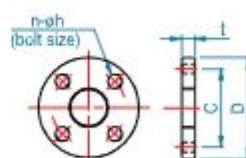
FLANGE DIMENSIONS (mm.)
