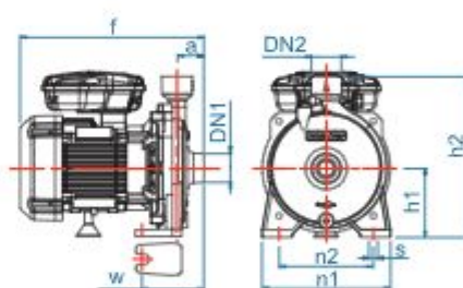
ACH-755S/ ACH-1105S
