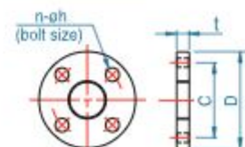
FLANGE DIMENSIONS (mm.)
