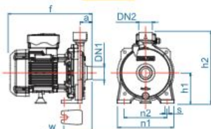
ACH-755T/ ACH-1105T
